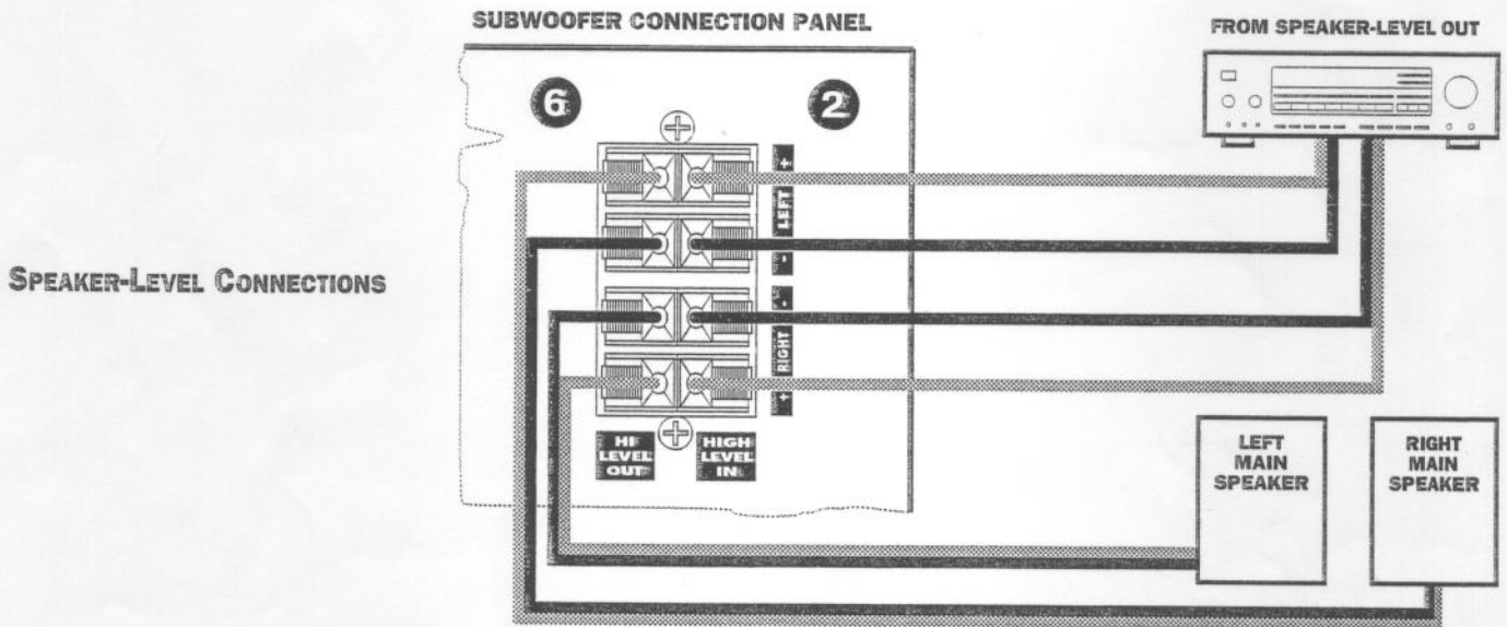
Figure 4. Connecting left and right speaker-level outputs of an A/V receiver to left and right speaker-level inputs of the subwoofer. Then connect left and right speaker-level outputs of the subwoofer, with the main left and right speakers of your system. Remember to maintain left to left, right to right, (+) to (+) and (-) to (-) connections.
