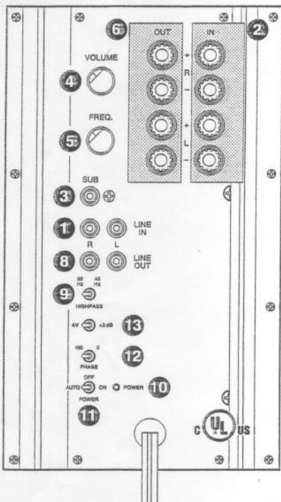
Figure 1. Connection panel for the HT-S15A and LW-15/15X.
