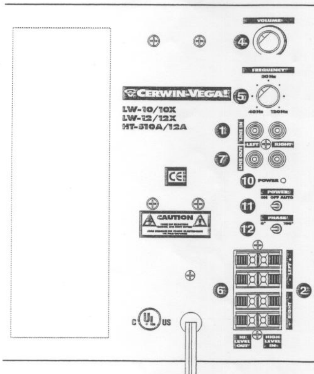
Figure 2. Connection panel for the HT-S10A, HT-S12A, LW-10/10X, and LW-12/12X.
